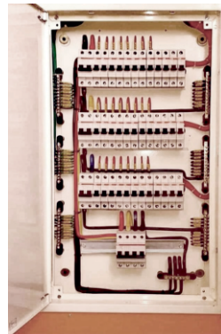
Distribution Board Installation on Site
